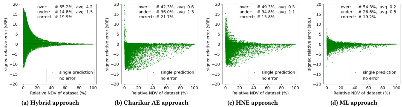
Figure 3: Prediction errors (sRE, eq. (21)) for the MLtrain dataset using i.i.d. samples ordered by the relative NDV of the datasets.
