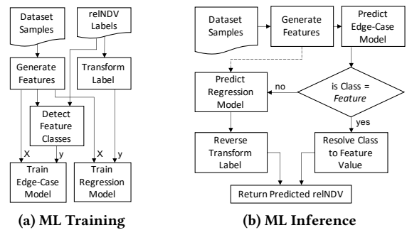
Figure 2: Training and inference for the ML approach.
