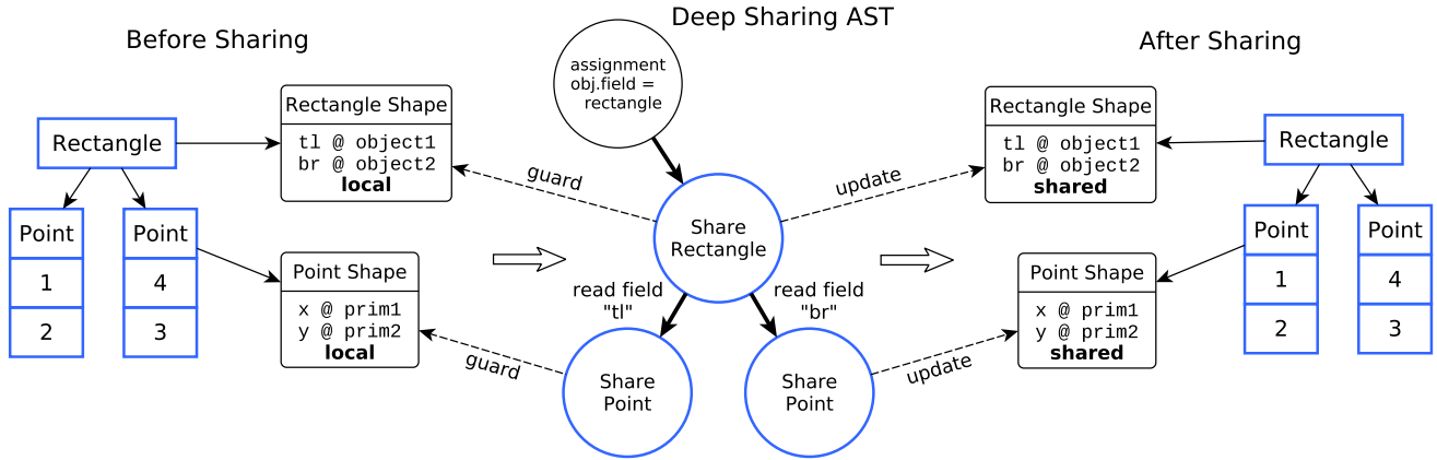
Figure 6. Deep Sharing of a Rectangle and two Points. The AST structure mirrors the one of the Rectangle and its Points. The Share nodes check if an object matches the expected shape and update it to a shared variant.
