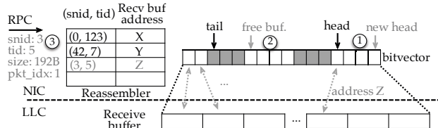
Fig. 5. NIC RPC reassembly and buffer management.
