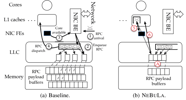
Fig. 3. Overview of baseline and NEBUA architectures.
